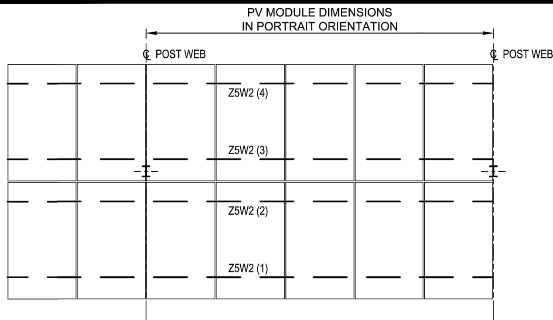
E3 5W2P2 SCALE: 1/4" = 1'-0" BAY PLAN VIEW
