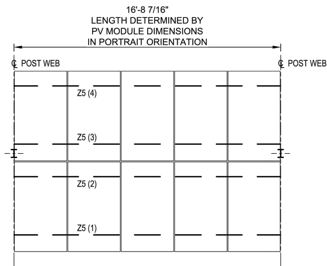
C3 5P2 SCALE: 1/4" = 1'-0" BAY PLAN VIEW
